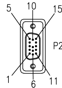
HDB15P/M
